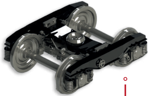
H-Type Bogie with Knorr Brake System
